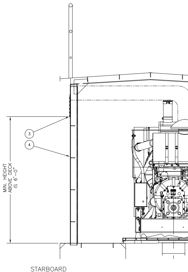
TYPICAL CROSS SECTION OF VOID VENTS N.T.S.
