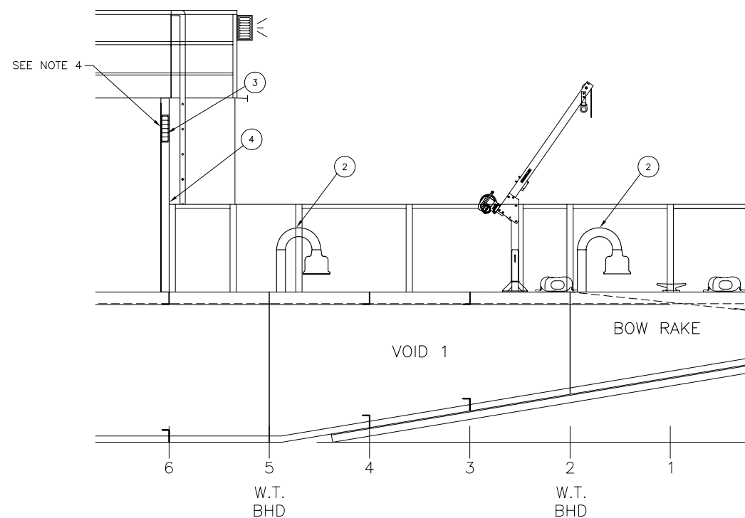
TYPICAL PROFILE OF VOID VENTS N.T.S.
