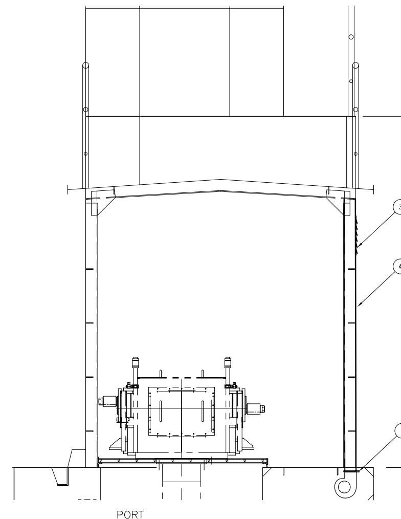
TYPICAL CROSS SECTION OF VOID VENTS N.T.S.
